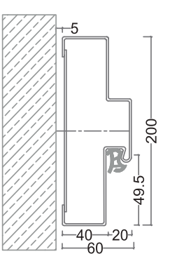
Standard: 200x60mm
