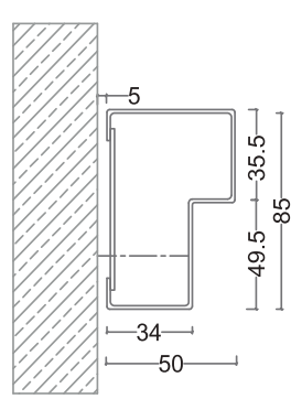
Standard: 85x50mm
