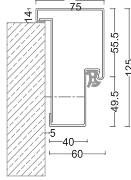
Architrave: 125x60x75mm
