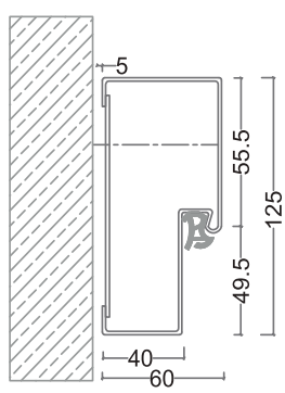
Standard: 125x60mm
